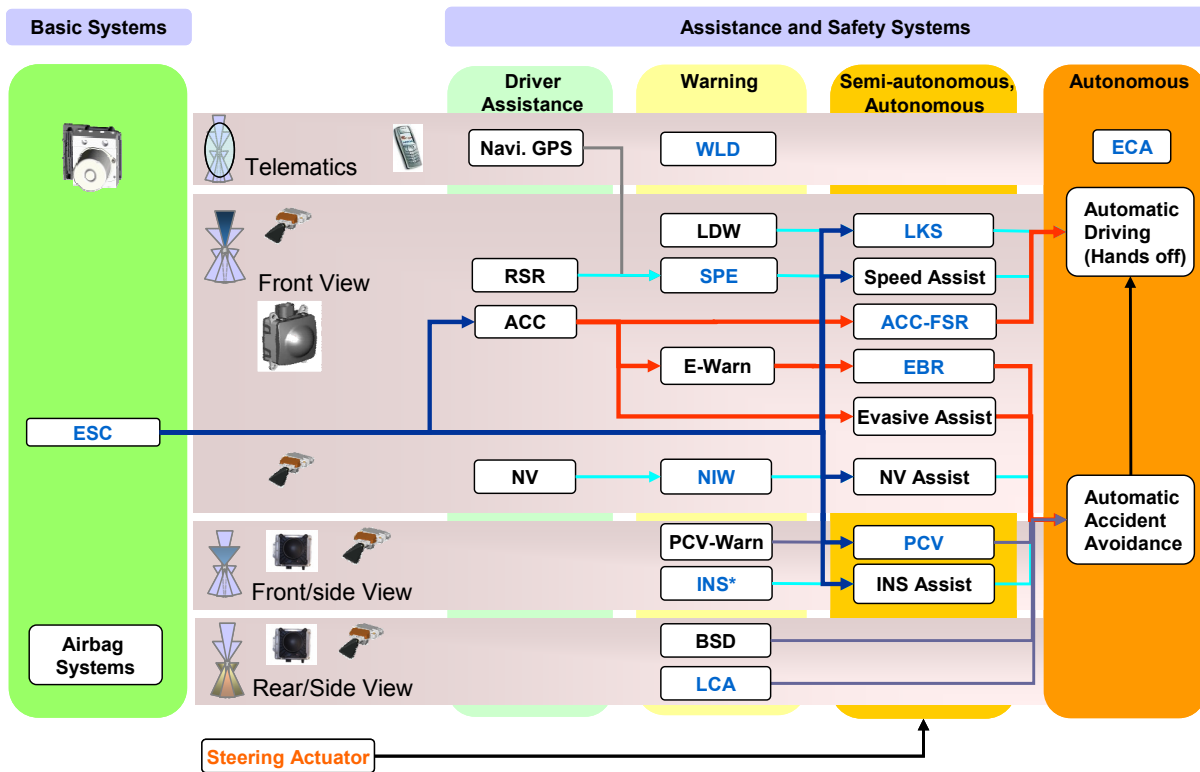
Figure 26: System dependencies
